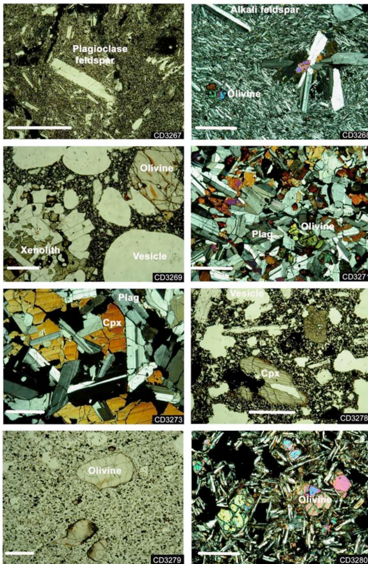
Figure 4. Photomicrographs of thin sections of some of the geological specimens collected by Darwin from the west of Isla Santiago. CD3267 (trachyandesite) and 3268 (trachyte) were collected during Darwin's trek into the Highlands. CD3269 and 3278 are vesicular basalts from Buccaneer Cove. CD3279 is a large feldspar basalt from a dyke at Buccaneer Cove. Specimens CD3271 (troctolite) and 3273 (gabbro) are 'coarse-grained fragments' (xenoliths) from Buccaneer Cove; and CD3280 is an olivine basalt from James Bay. Images of CD3267, 3269, 3278 and 3279 were taken in plane-polarized light. Images of all other samples were taken using cross-polarized light. The scale bar in the bottom left-hand corner of each image is 1 mm. Brief descriptions of the samples are given in Table 2. (Images by courtesy of S.A Gibson.)
